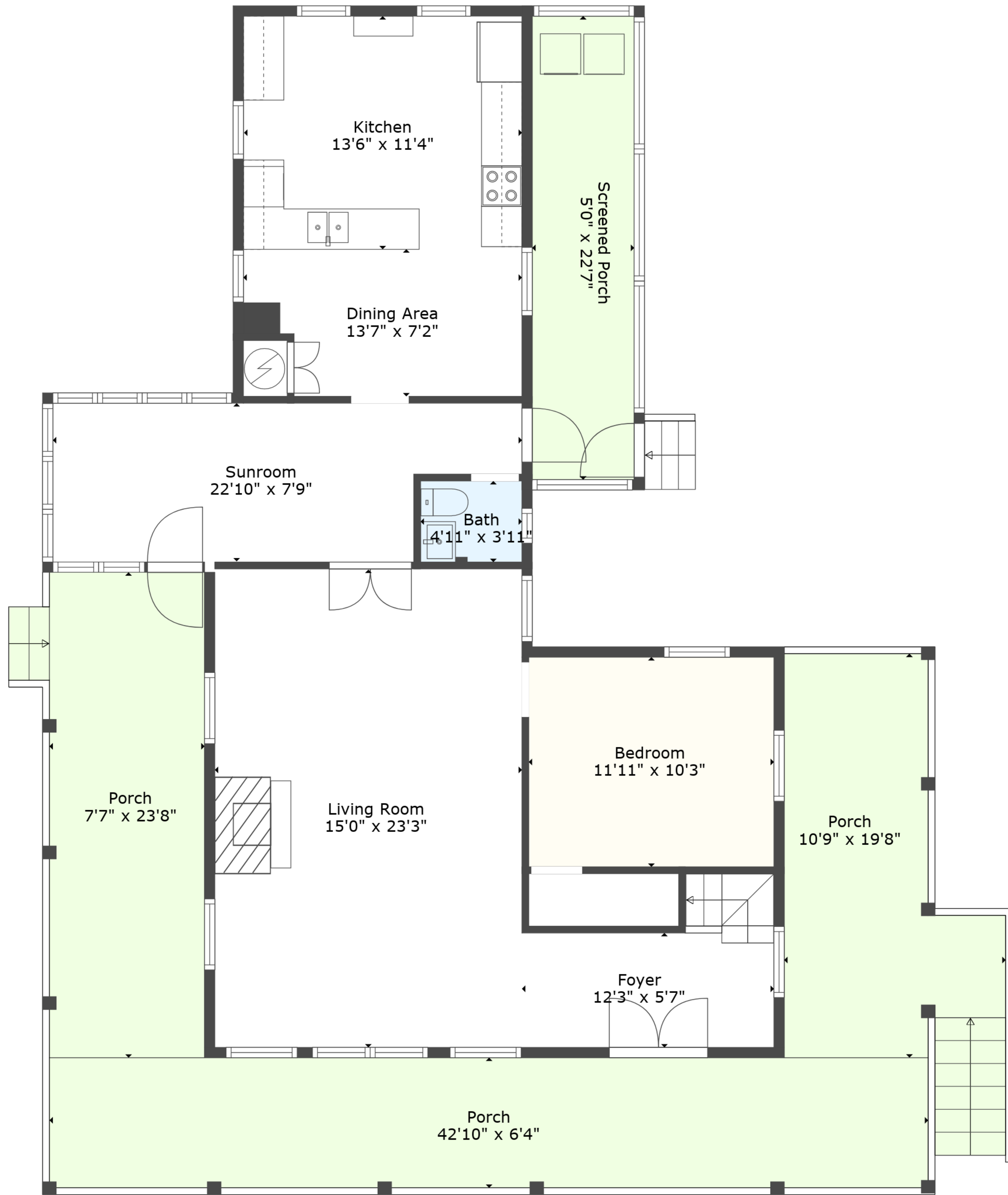
Floor 1
